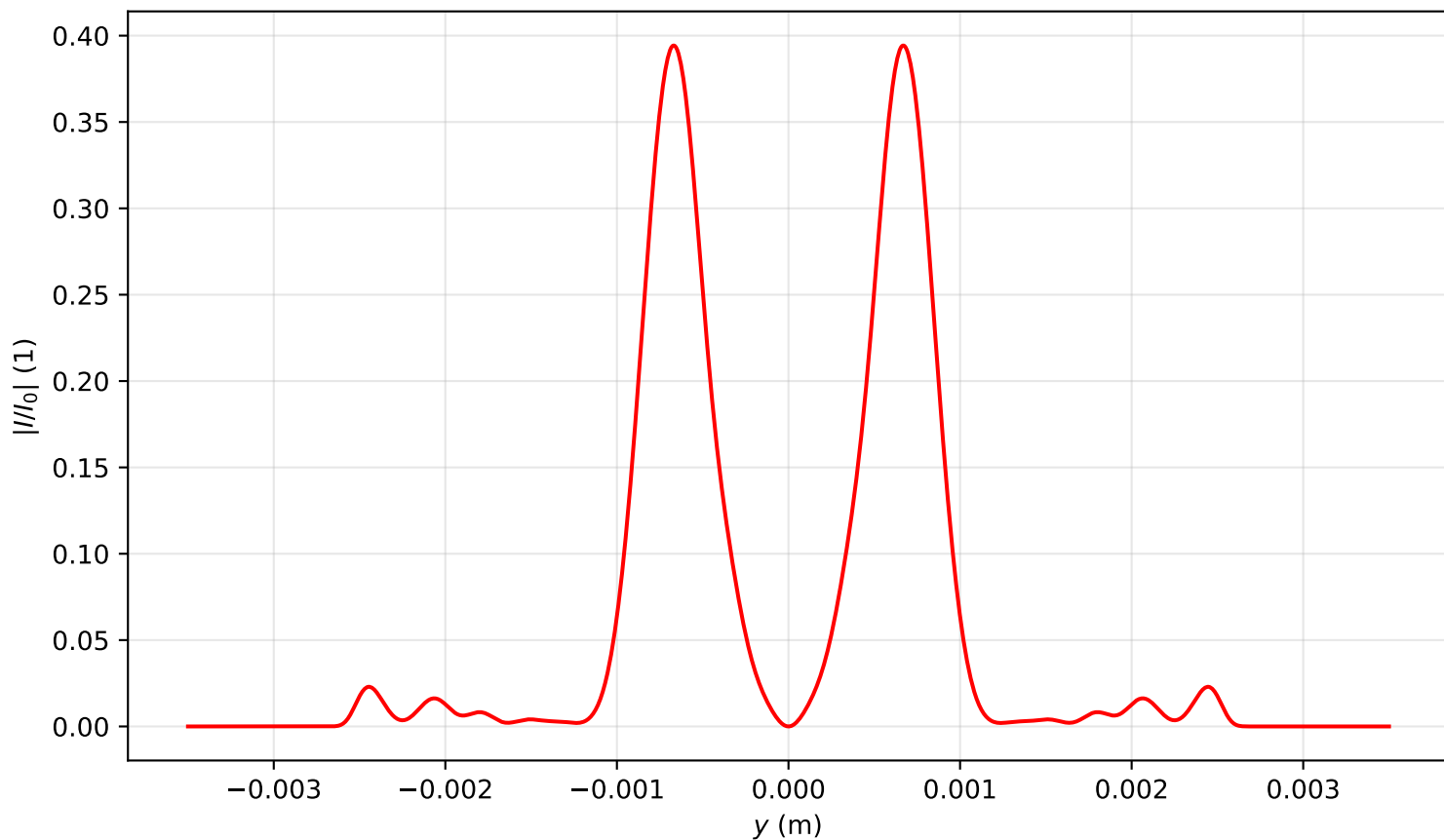
Intensity profile I(x=0, y, z=2.309)/I_0 , \text{Pin}=7.0\text{Pcr} , artificial time
